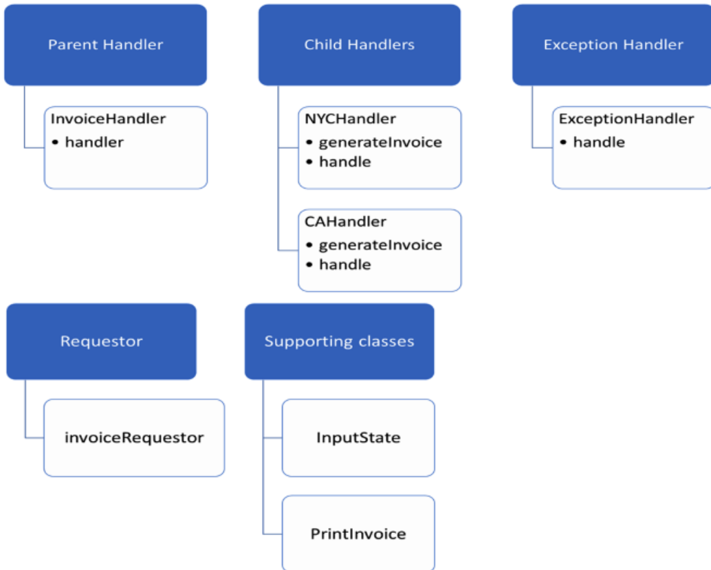
Figure 12.1 – Chain of responsibility classes
