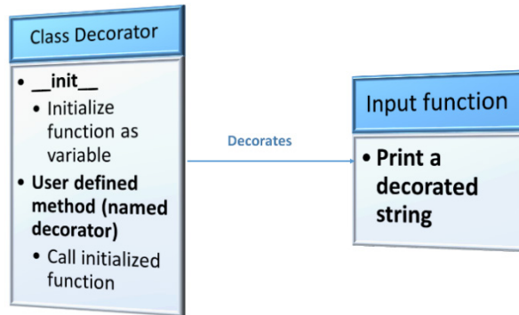
Figure 3.7 – Wrong method for creating a class decorator
