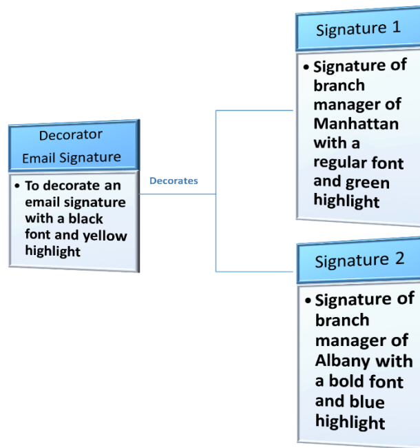
Figure 3.1 – Email signature decorator
