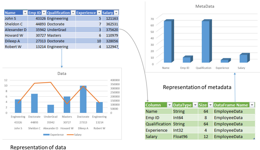
Figure 1.2 – Metadata representation for the Employee Data table
