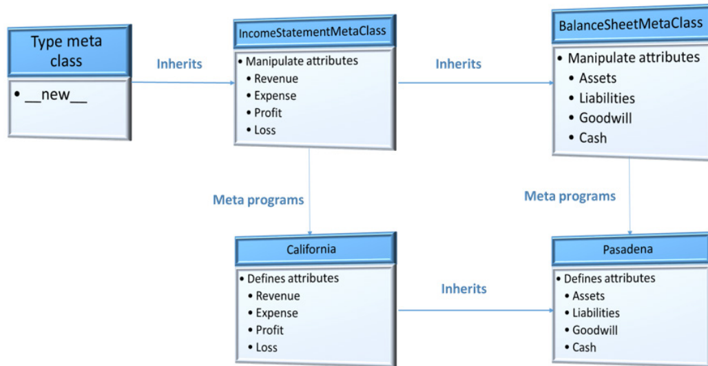
Figure 4.11 – Inheritance in metaclasses
