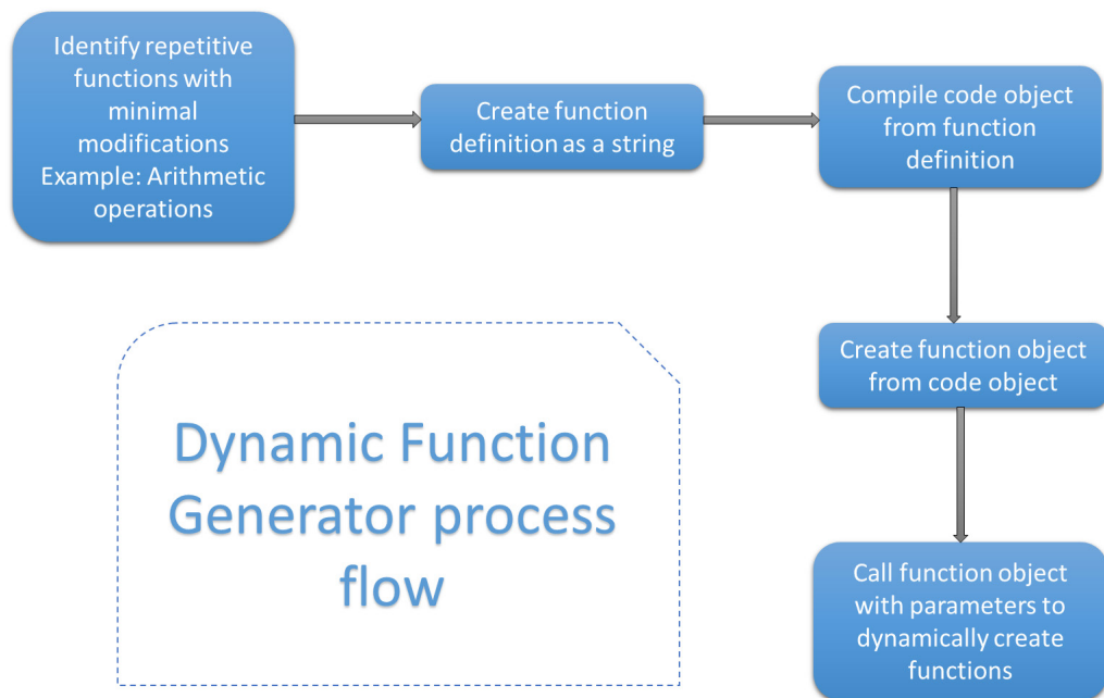
Figure 1.8 – Dynamic function generator
