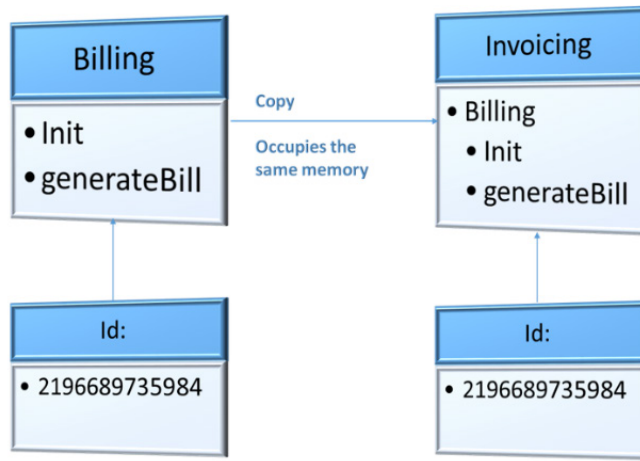
Figure 5.2 – Two classes with one memory address
